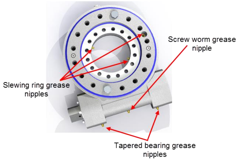
Image 2: Explanation on the grease nipples of the slew drive
